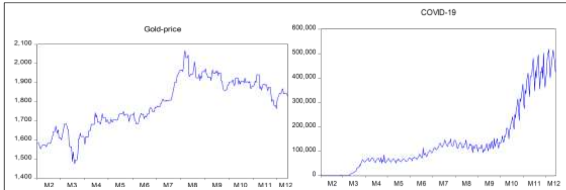
Figure (1): Time Series Plots of the Variables (R-Studio v.4.5.1)
